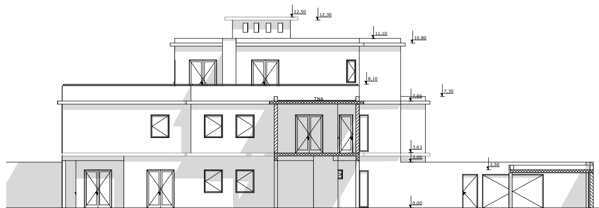
FACADE SUD
